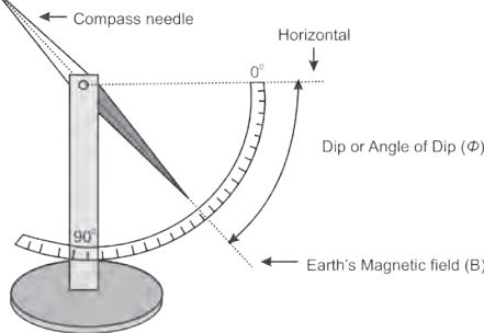
Fig. 12.7: Magnetic inclination.
