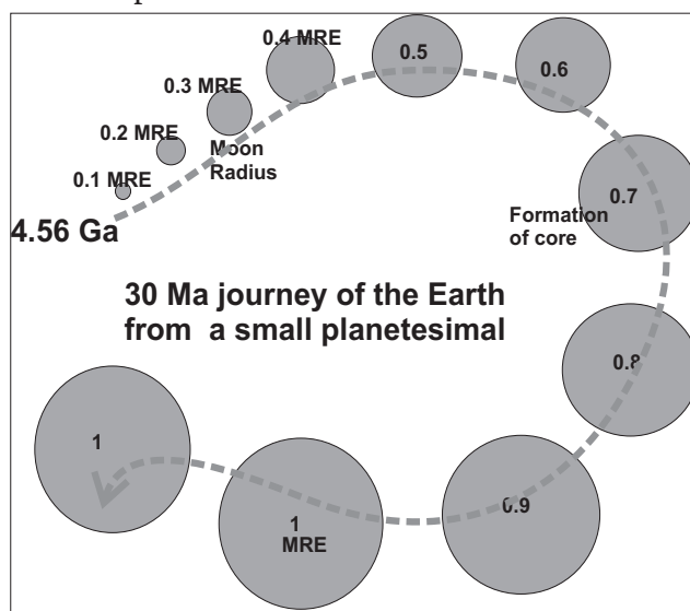
Fig. 1.1 : Evolution of the Earth from a planetesimal state
